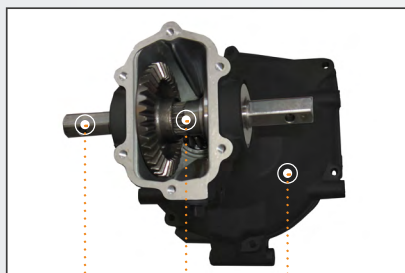
Carter fresa in ghisa
